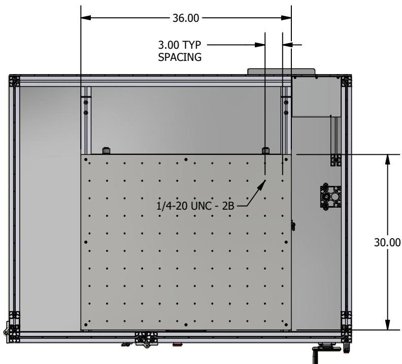
SECTION C-C FIXTURE MOUNTING PLATE
