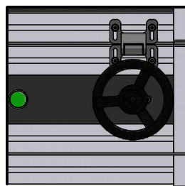
DETAIL A LASER HEAD HEIGHT ADJUSTMENT WHEEL AND TRIGGER BUTTON
