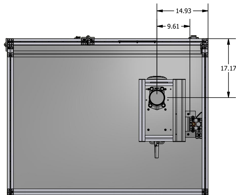
SECTION D-D LASER HEAD MOUNT & INTERNAL LIGHTING
