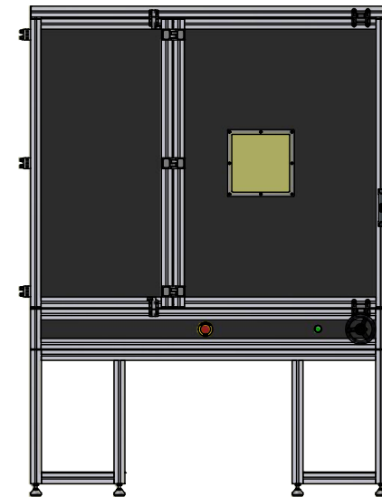
DOORS OPEN WITH MOUNTING PLATE EXTENDED
