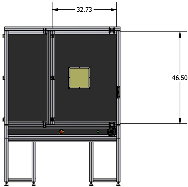
RIGHT DOOR OPEN (PRIMARY)
